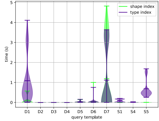
Figure 10. The termination time distribution by query template. With the exception of queries from templates D6 and D7, which have similar execution times, the shape index either maintains or improves query termination time.
