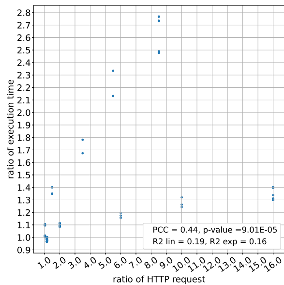
Figure 15. Shape index approaches tend to perform less effectively with limited network information and comparatively better where the baseline shape index underperforms. A higher ratio indicates a longer query execution time compared to a network with complete shape index information ( lower is better ).
