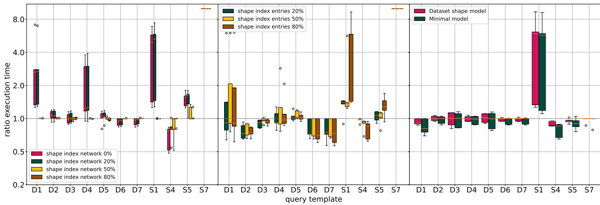
Figure 15. Shape index approaches tend to perform less effectively with limited network information and comparatively better where the baseline shape index underperforms. A higher ratio indicates a longer query execution time compared to a network with complete shape index information ( lower is better ).
