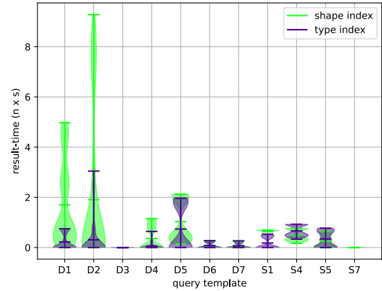
Figure 13. The dief@1s distribution by query template. At 1 second, the shape index approach shows a higher dief@1s (higher is better), indicating that more results can be obtained by users while maintaining a seamless flow of thought.
